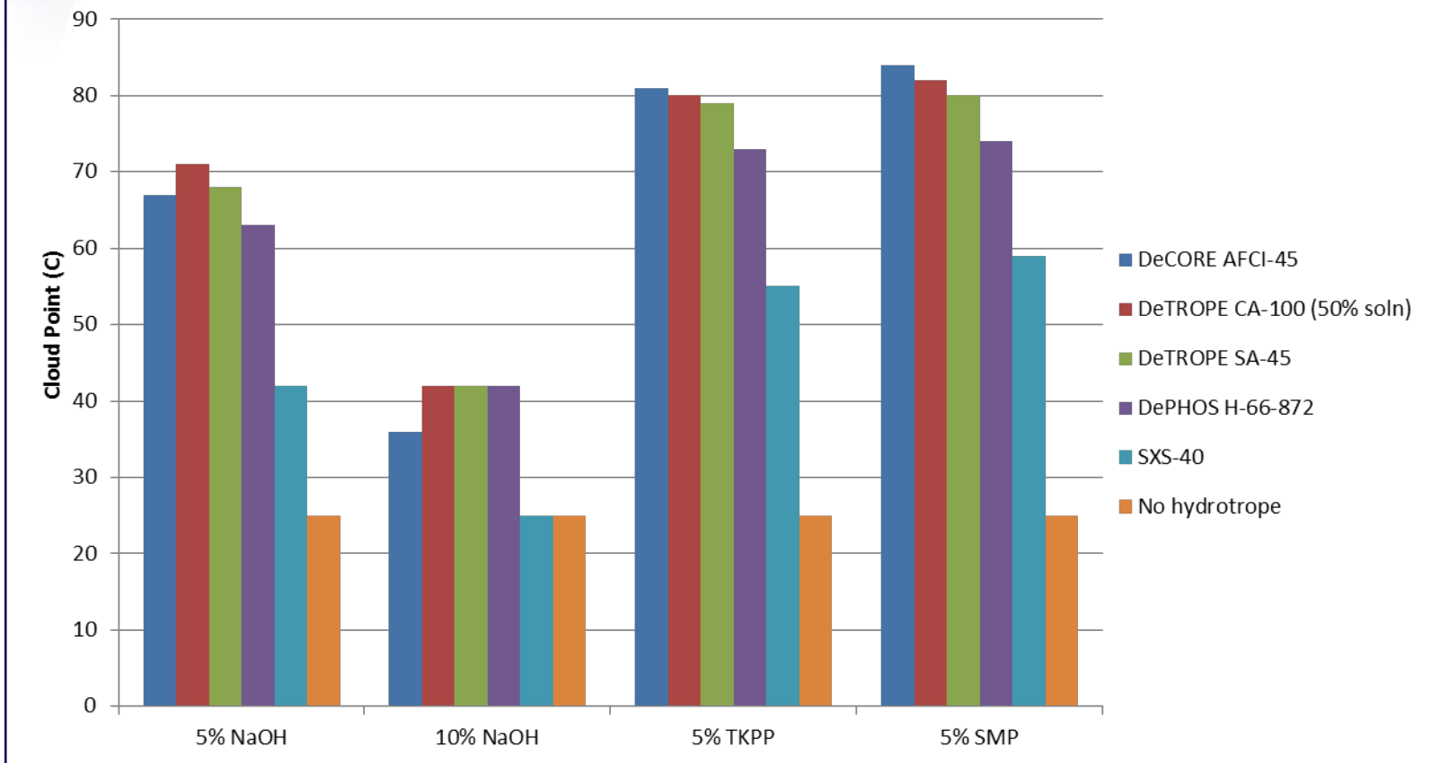
Cloud Points of Test Solutions: 5% NPE-9, 3.75% Hydrotrope (by wt.), 91.25% Electrolyte
