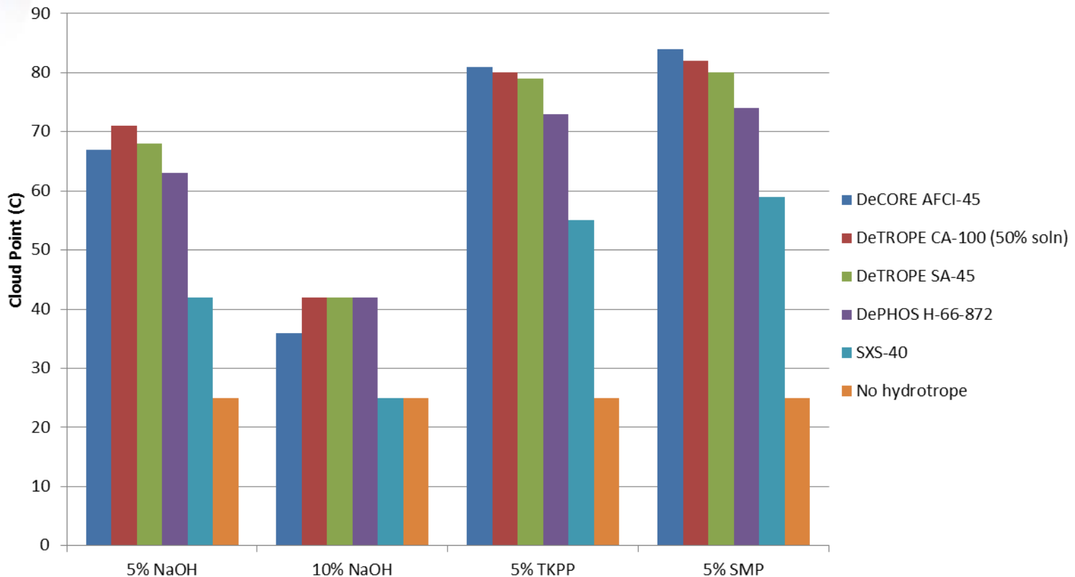
Cloud Points of Test Solutions: 5% NPE-9, 3.75% Hydrotrope (by wt.), 91.25% Electrolyte
